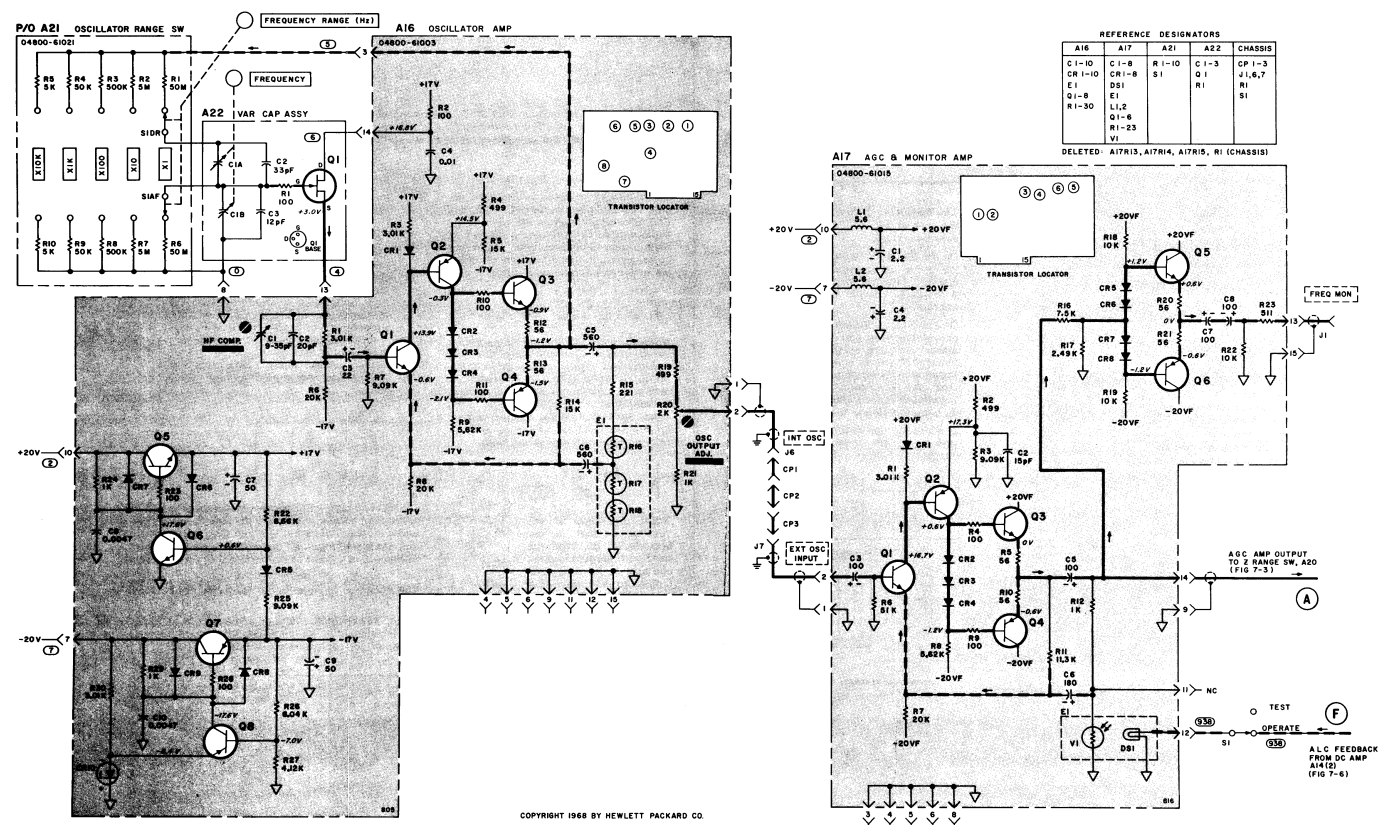
Figure 7-2. OSCILLATOR-AGC AMPLIFIER
